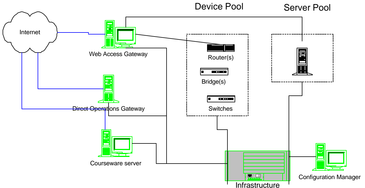
Figure 1 ARMS Overview
